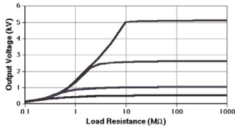
Typical Terminal Voltage Characteristics
